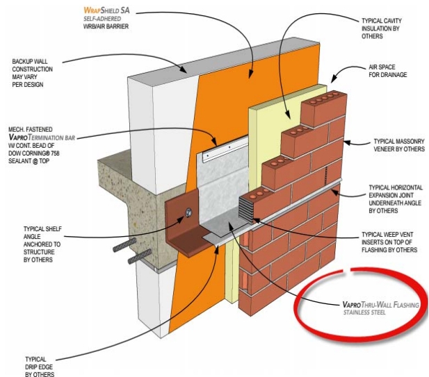
SHELF ANGLE DETAIL with VaproThru-Wall Flashing SA™ Self-Adhered Stainless Steel & VaproTermination™ Bar
